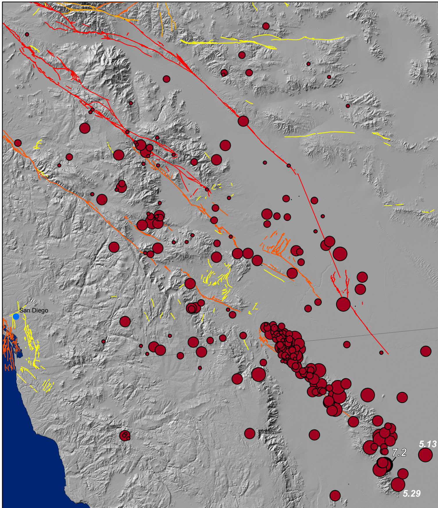
Fault slip rate (mm/yr) Main shock and ~12 hours seismicity/aftershocks Baja California
