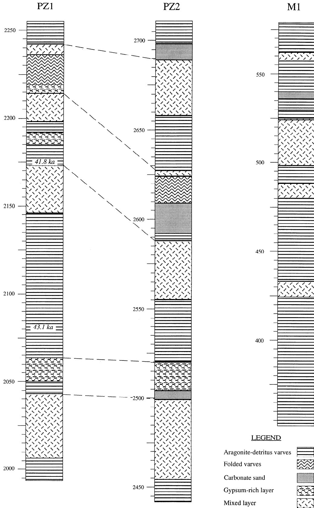
Figure 8. An example of segments of sections PZ1 and PZ2 in the Peratzim Valley and M1 near Masada. The level is measured in centimeters from the base of the Lisan Formation. Detailed correlation is hindered by facies variations. We suggest a tentative correlation between PZ1 and PZ2, which will be tested by radiometric dating.
