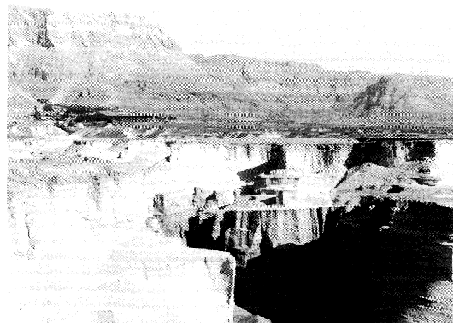
Figure 2. Typical view of Lisan Formation. The hard, gypsum-rich top of the formation forms a flat plain unaffected by syndepositional faults. Vertical exposures are about 40 m.
